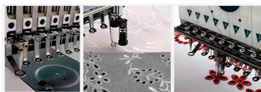
Boring Device 雕孔针
